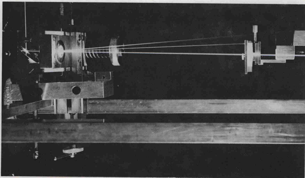
Fig. 11. Apparatus Used in Laser Raman-High Pressure Experiment.
